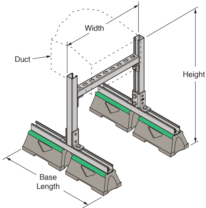
DSACBN-DSF Duct Support Series With Fixed Width & Adjustable Height
