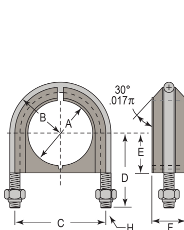
1/2" thru 6" assembly.
